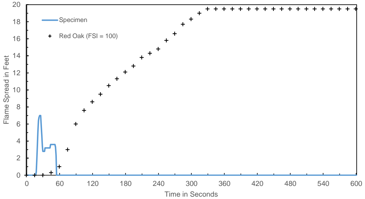
Chart 1. FLAME SPREAD
