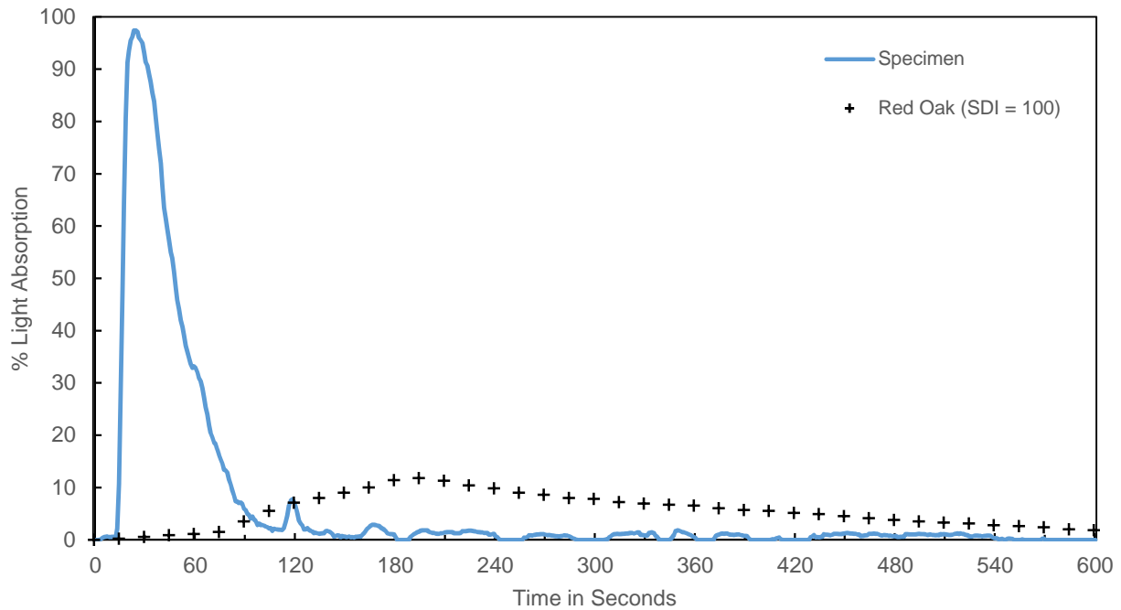
Chart 2. SMOKE DEVELOPED
