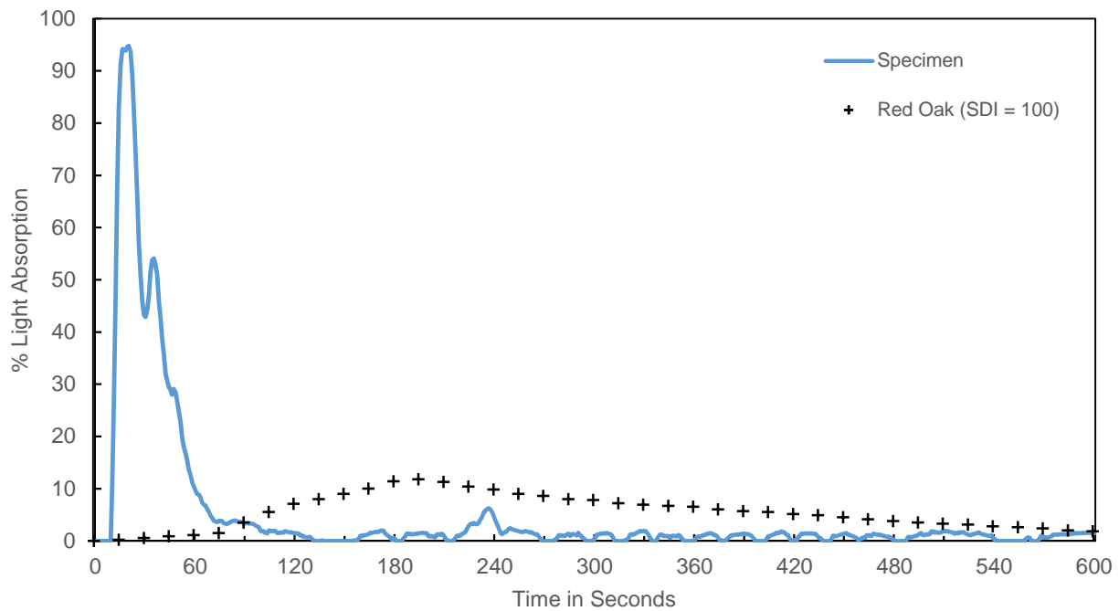
Chart 2. SMOKE DEVELOPED
