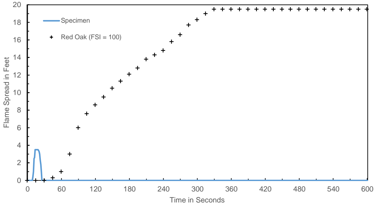
Chart 1. FLAME SPREAD
